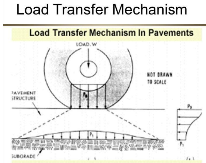
Figure 4 : Load transfer in rigid pavemet
