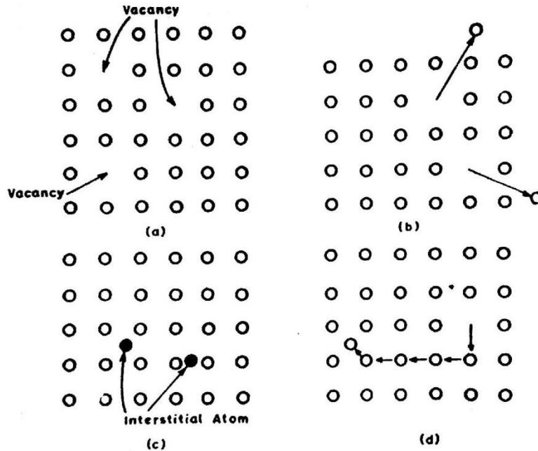
Fig 3.5 Various types of point defects. (a) Vacancy, (b) Schottky defect, (c) Interstitialcy, (d) Frenkel defect. Types and causes of line defects, Edge dislocation and screw dislocation.
